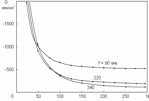
Figure 2. Conductance as function of period number N.
