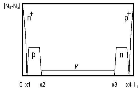
Figure 1. Doping profile for DAR IMPATT diode.
