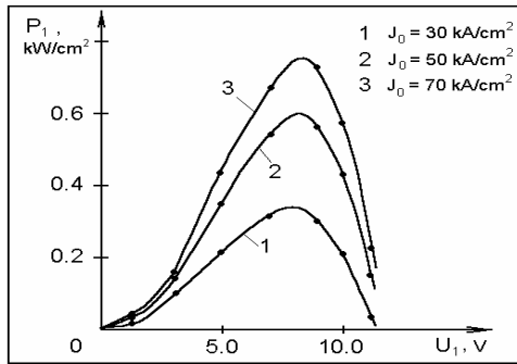
Figure 6. Output generated power P dependency as functions of first harmonic amplitude U_1 for 220GHz.
