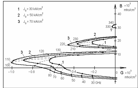
Figure 4. Complex small signal DAR diode admittance optimized for second frequency band for different value of feeding current.
