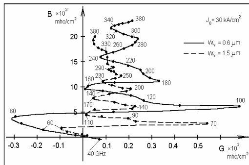
Figure 3. Complex small signal DAR diode admittance for different frequencies and two values of drift layer widths W_v .
