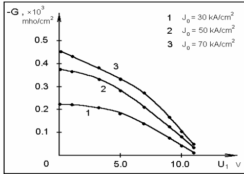
Figure 5. Conductance G dependency as functions of first harmonic amplitude U_1 for 220 GHz.
